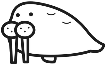
walrus
