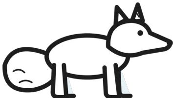
arctic fox
