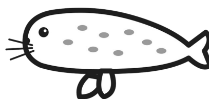
Weddell seal
