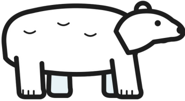
polar bear
